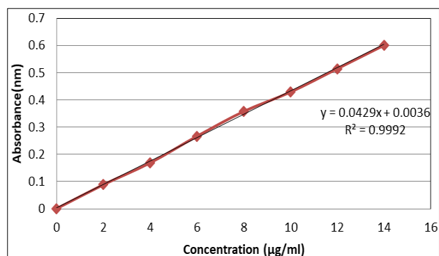
Fig 3: Calibration Curve of Lornoxicam
