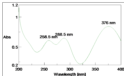
Fig 2: A typical UV Spectrum of Lornoxicam at 376 nm
