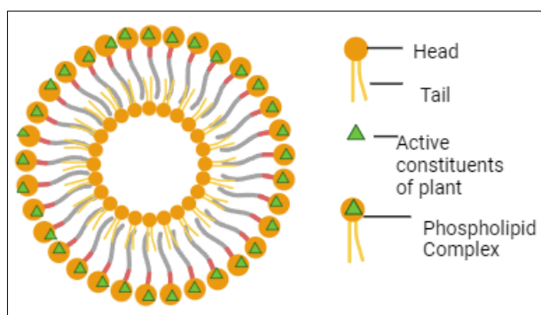
Fig 1: Phytosome Structure
